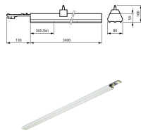
Technische Daten Philips LED Tragschiene Coreline LL234X 56W 9000lm 67x67D - 840 | 3400mm - 5-polig
